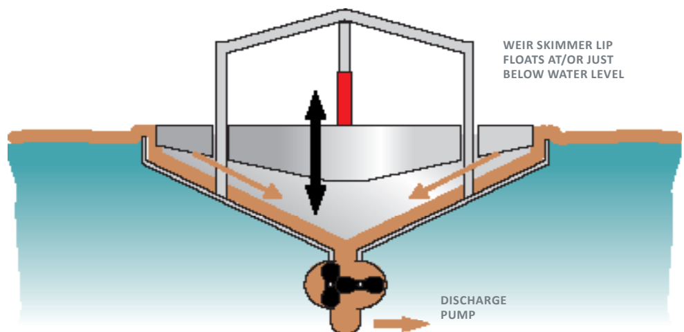
Weir skimmer diagram
